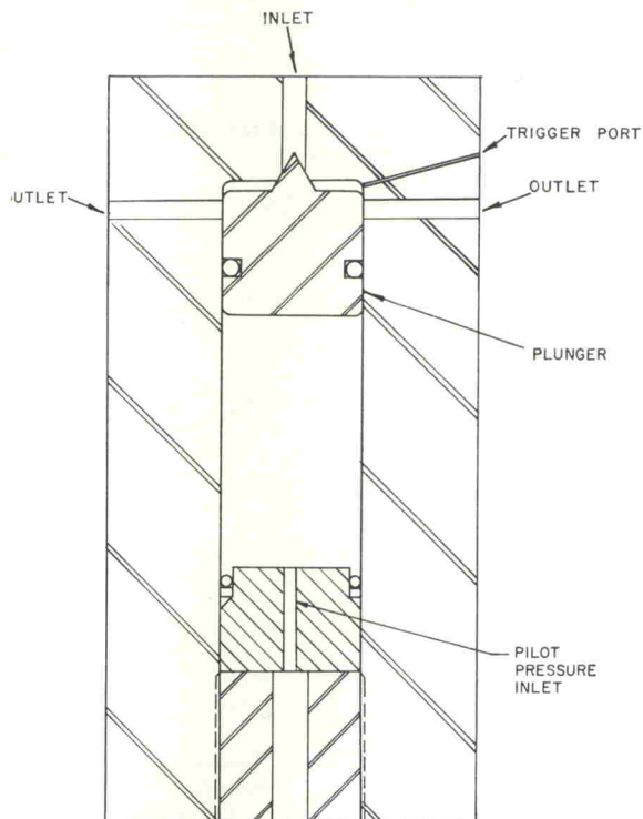
Fig. 3.—Schematic of high-speed valve.
